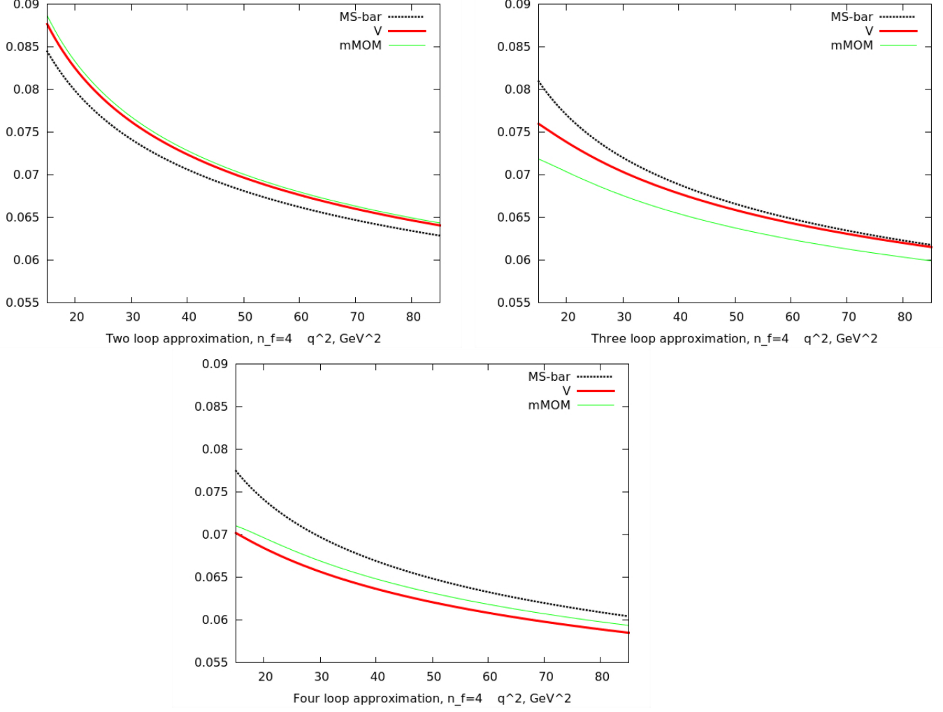
FIG. 1: Scheme dependence of the NLO (left), NNLO (right) and N^3\text{LO} (bottom) approximations for the e^+e^- characteristic r(q^2) = R(q^2)/(3\sum_f Q_f^2) - 1 in the case of n_f=4 numbers of active flavours. The dashed black curve depicts the variations of the \overline{\text{MS}} approximants. The solid (green) line demonstrate the variations of the mMOM-scheme results, while the solid red line shows the V-scheme results.
