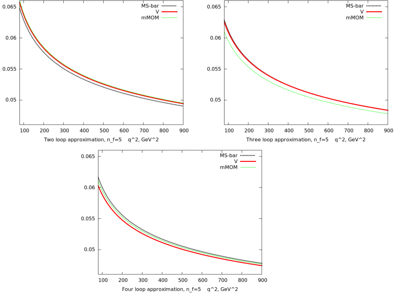
FIG. 2: Scheme dependence of the NLO (left), NNLO (right) and N 3 LO (bottom) approximations to r(q^2) are presented for n_f=5 numbers of active flavours. The variation of the \overline{\text{MS}} -, mMOM- and V-scheme results is indicated by the three curves as in Fig.1
